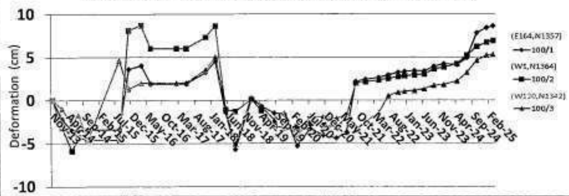
MOVEMENT : MONITORING TREND OF WASTE DUMP AT 100m LIFT BY PRISMS
