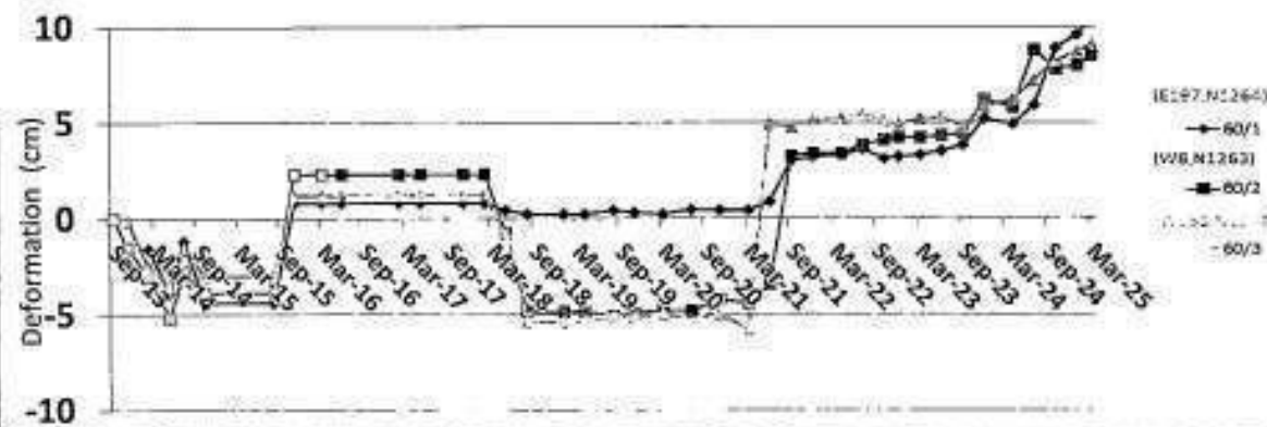
MOVEMENT: MONITORING TREND OF WASTE DUMP AT 60m LIFT BY PRISMS
