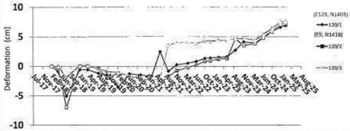
MOVEMENT : MONITORING TREND OF WASTE DUMP AT 120m LIFT BY PRISMS
