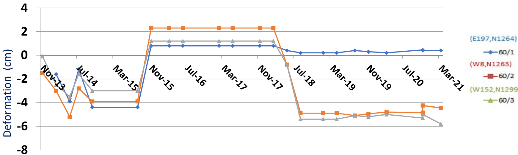
MOVEMENT: MONITORING TREND OF WASTE DUMP AT 60m LIFT BY PRISMS
