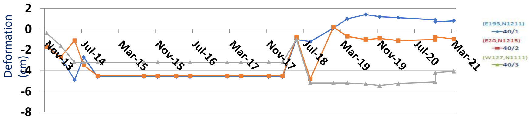
MOVEMENT : MONITORING TREND OF WASTE DUMP AT 40m LIFT BY PRISMS
