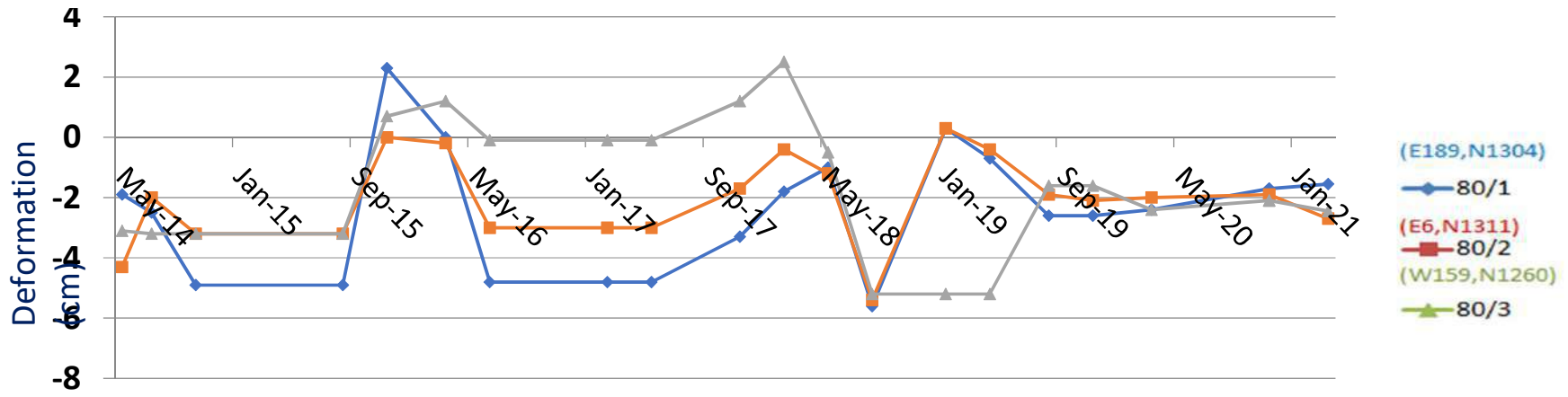
MOVEMENT: MONITORING TREND OF WASTE DUMP AT 80m LIFT BY PRISMS
