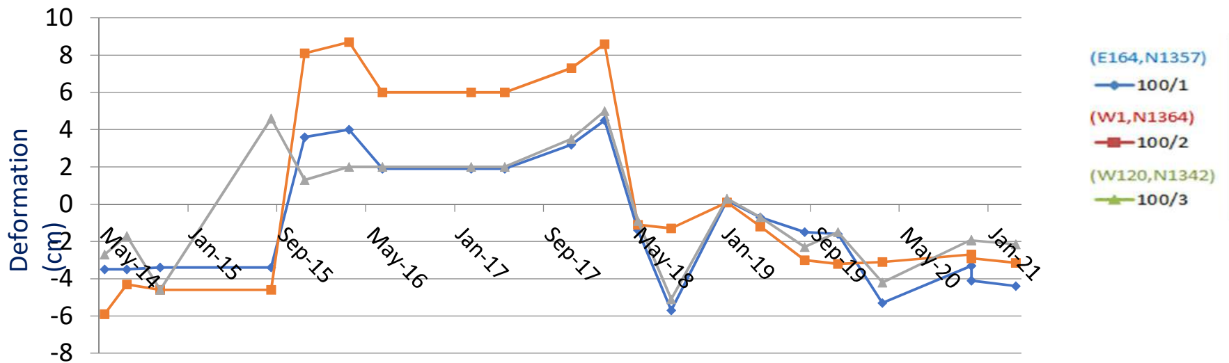
MOVEMENT : MONITORING TREND OF WASTE DUMP AT 100m LIFT BY PRISMS
