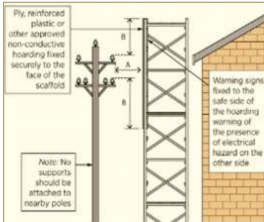
Figure 55: Non-conductive Hoarding for Scaffolds
