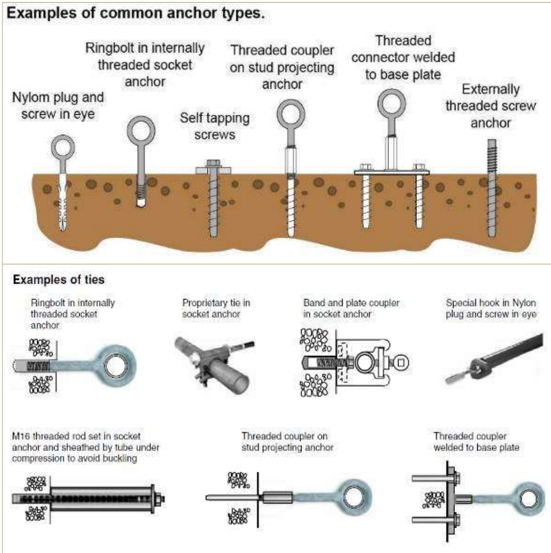
Figure27: CommonTypesofEmbeddedAnchorsandTieMethods
