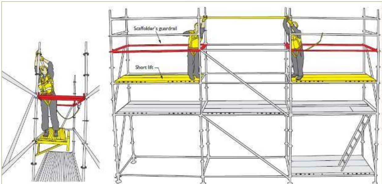
Figure 68: Systemscaffolds slide brackets used to create scaffolders' step platform in alternate bays. The middle bays can be reached from adjacent bays to fix the guardrails
