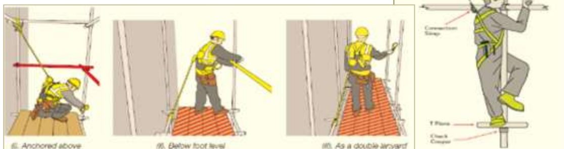
Figure 45: Examples of a hybrid self-retracting lanyard system in various scaffolding applications
