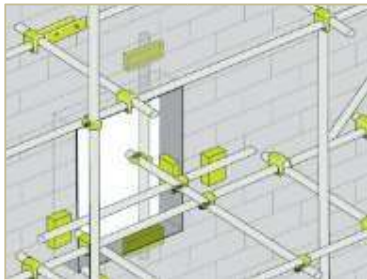
Figure 20: Lip/Opening Tie
