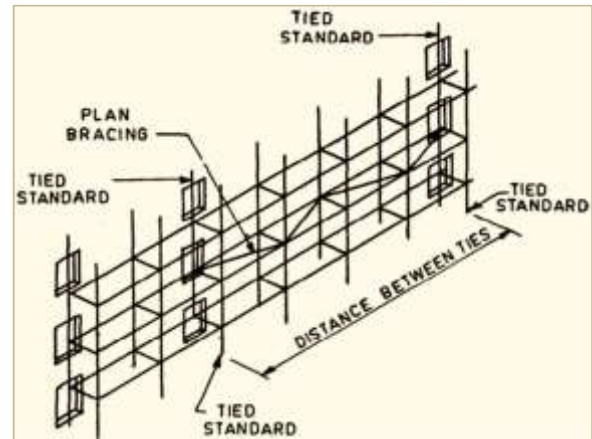
Figure 17: Plan Bracing
