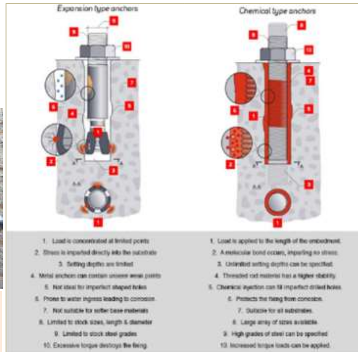
Figure28: ComparisonofExpansionTypev/sChemicalAnchors
