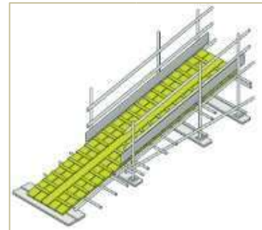
Figure 53: Barrow Ramp
