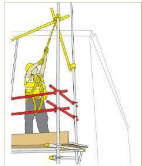
Figure 69: Pus type Advanced Guardrail Tool (AGT) using special couplers and a positioning tool
