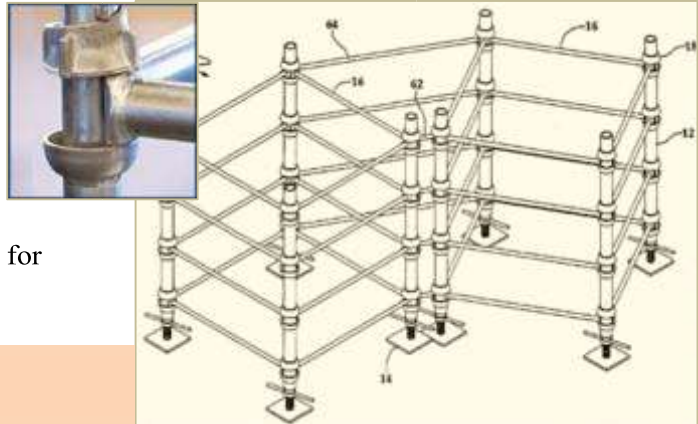
Figure 60: Cup-lock system
