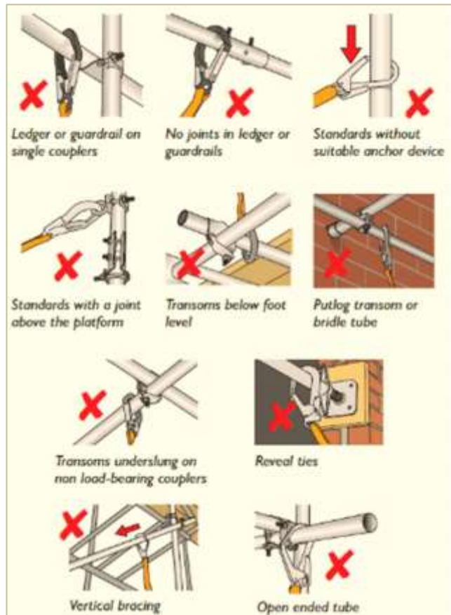
Figure 46: Examples of unsuitable anchor points
