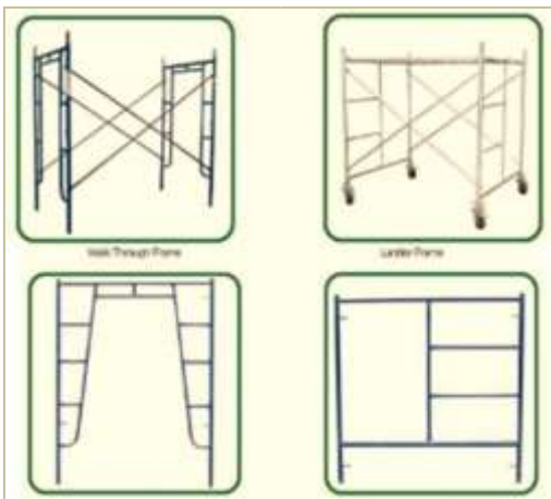
Figure65: Frameandbracescaffolding
