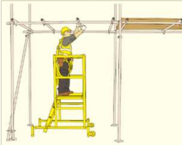
Figure 92: Scaffolders' Safe Zone in case of tall lifts (1) Scaffolders using scaffolders' steps to form a floor height; and (ii) Podium used as an alternative for taller lift heights
