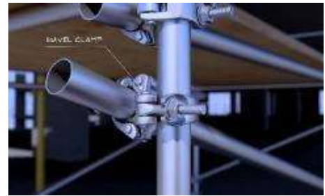
Figure2: Tube&CouplerScaffold
