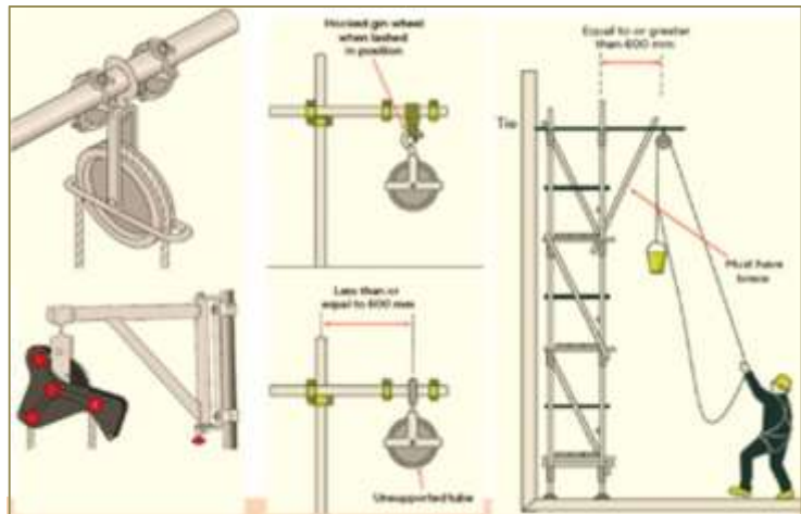
Figure30: GinWheels-Varioustypes
