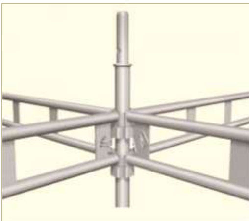
Figure 62: HAKI Scaffolding
