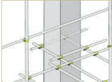
Figure 21: Box Tie
