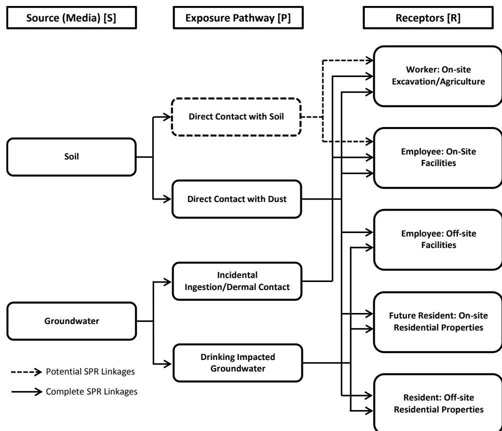
Figure A.5.2 Example of a Conceptual Site Model
