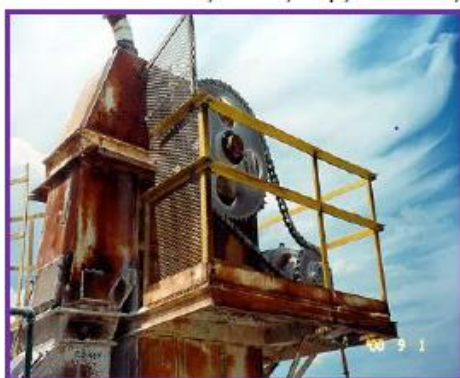
The sprocket and chain in this picture are not effectively guarded.
